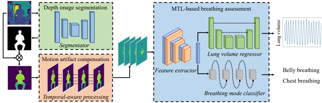
Fig. 2. DeepBreath overview.
